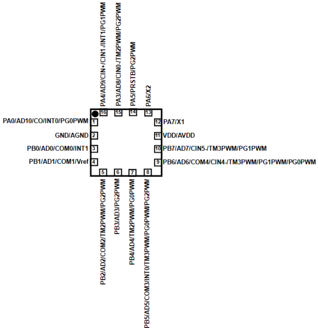
PFS173-1J16A (QFN3*3-16P-0.5pitch)
